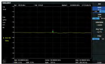
-165 dBm/Hz Displayed Average Noise Level
