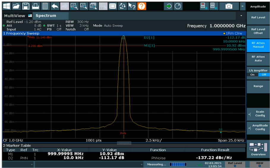
Phase noise at 10 kHz from the carrier: -137\text{ dBc} (1 Hz).
